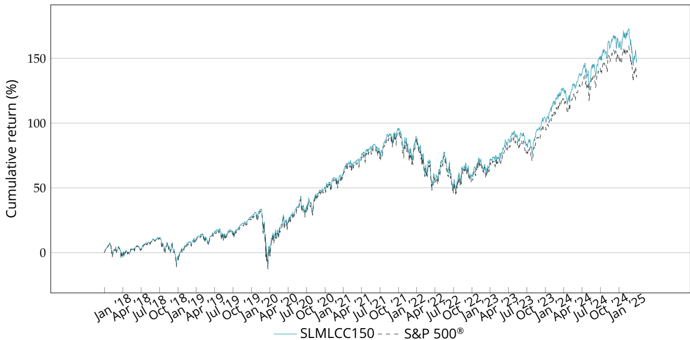
Historical Performance (12/29/2017 – 03/31/2025)
